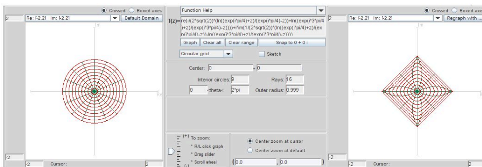
FIGURE 4.24. Image of \mathbb{D} under f_2
