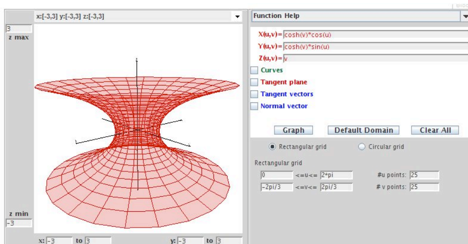
FIGURE 2.18. The catenoid.
