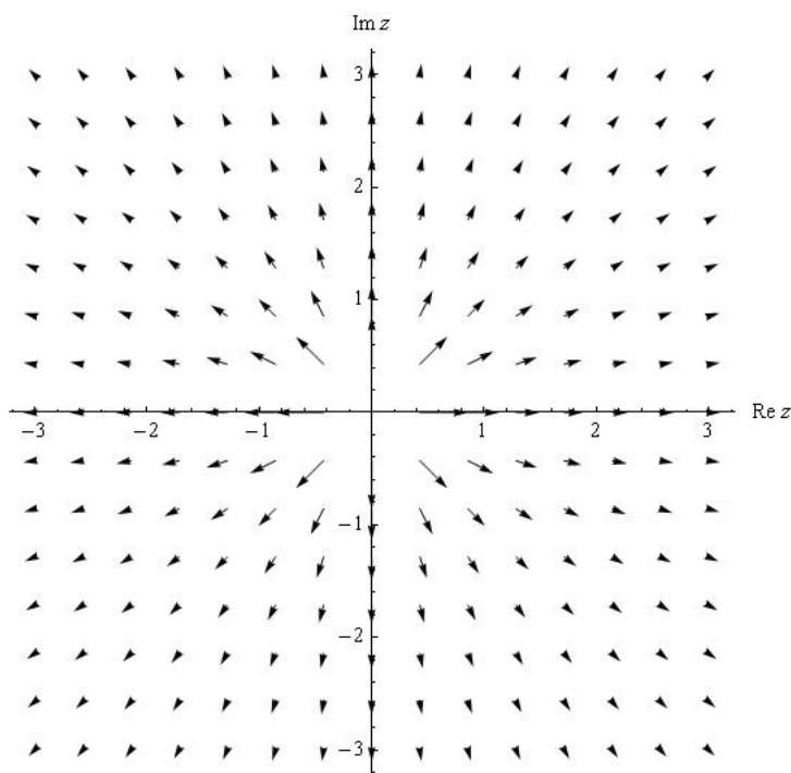
FIGURE 3.7. Polya vector field of the analytic function f(z) = \frac{1}{z}
